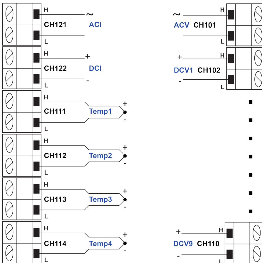
Figure 42: 7700 channel connections
