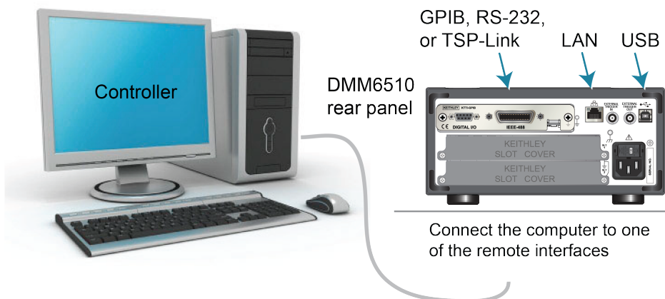
Figure 16: DAQ6510 remote interface connections
